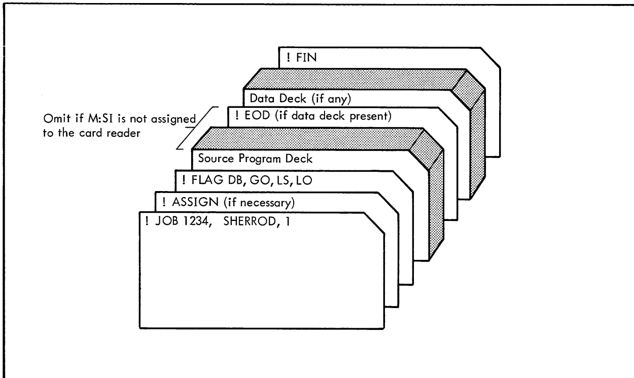
Figure 3. FLAG Job Setup – Single Program
