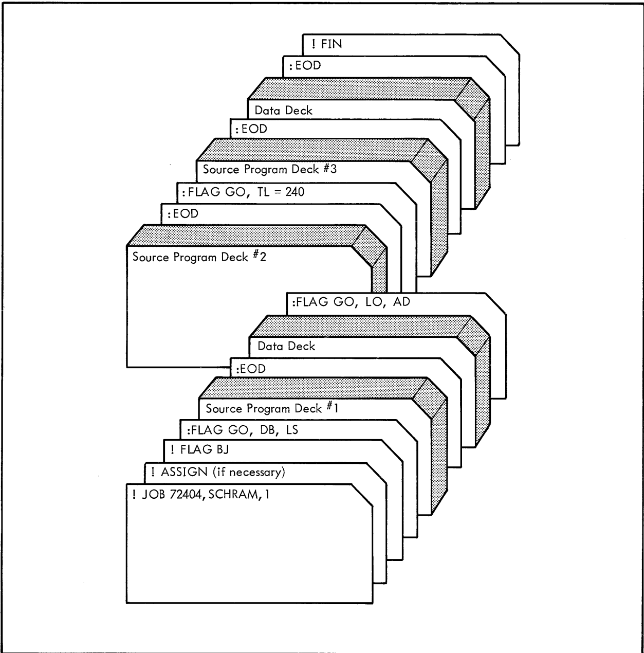
Figure 4. FLAG Job Setup – Multiple Programs in Batch Processing Mode
